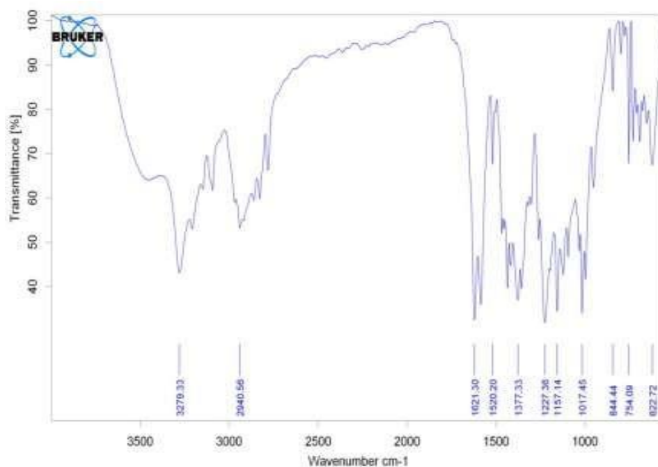
Figure 7: FT-IR spectrum of Nizatidine + HPMC K15M+ Sodium alginate
