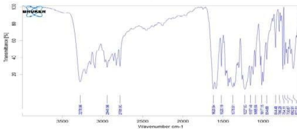
Figure 1. FT-IR spectrum of Nizatidine pure drug
