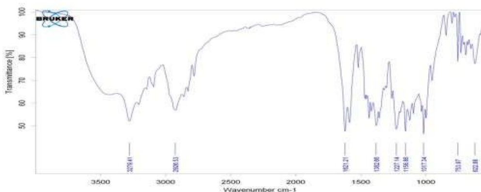
Figure 2: FT-IR spectrum of Nizatidine + HPMC K4M+ Sodium CMC
