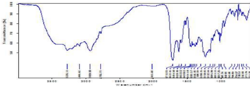
Figure 3: FT-IR spectrum of Nizatidine + HPMC K4M +Carbopol 934P
